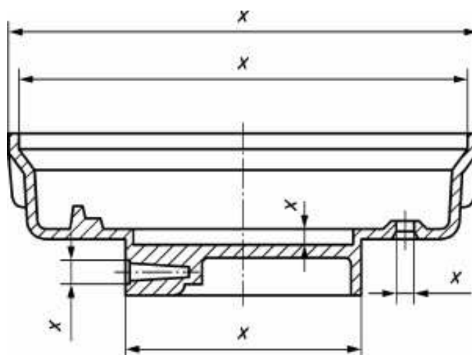
Figure 1 — Tool-specific dimensions
